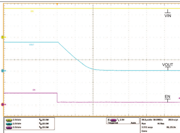
V IN = 5 V, C OUT = 1 μF, R ILM = 487 Ω
